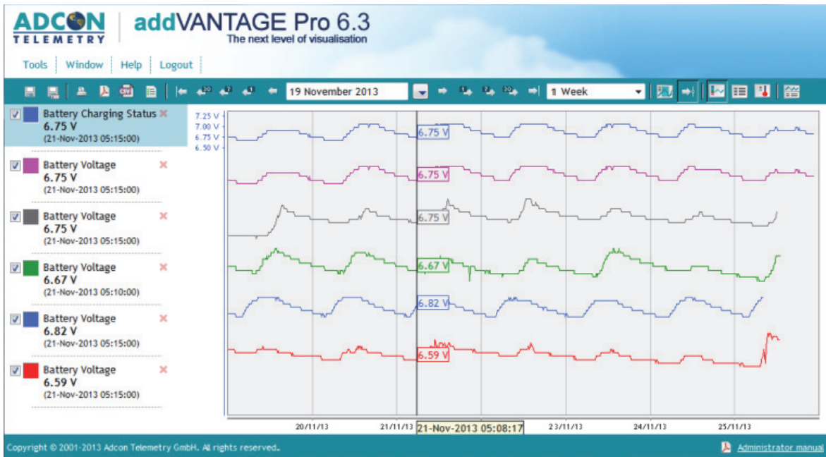
Figure 40. A Trend Viewer Showing Tags from Several RTUs
